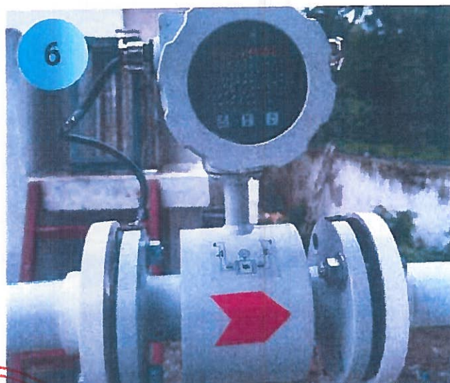
Flowmeter Installed
